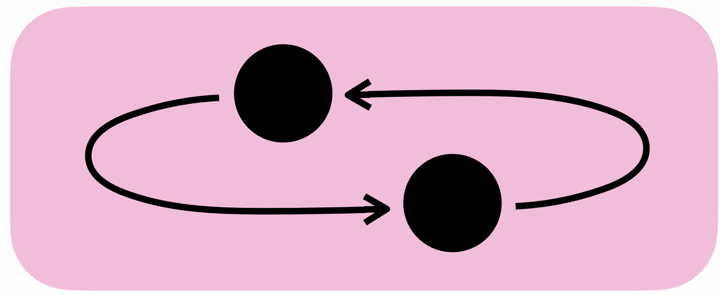
Black hole mergers
