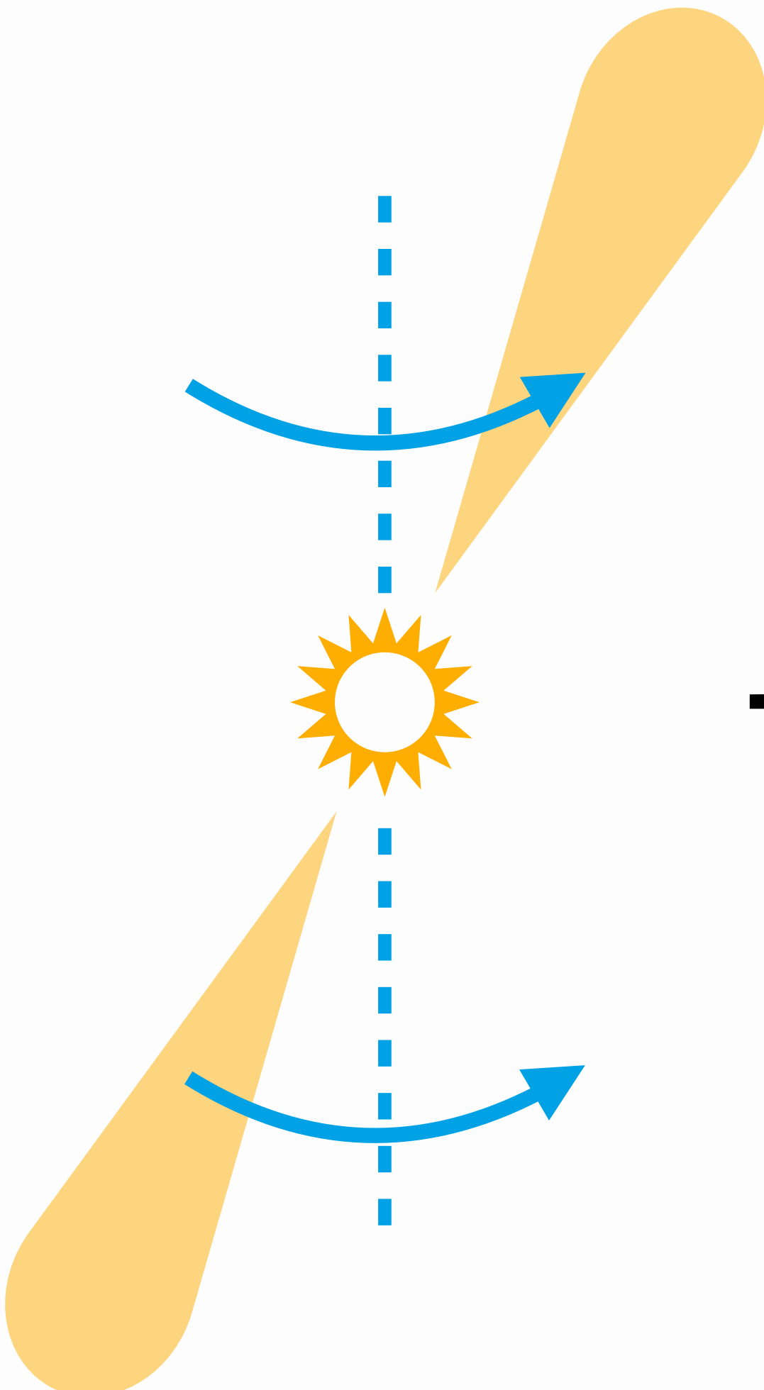
Pulses expected from timing model
