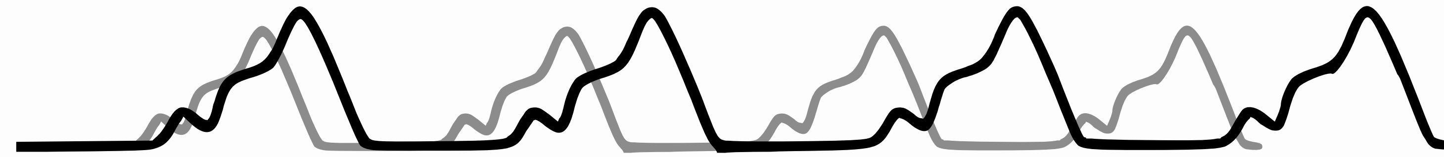
Pulses expected from timing model
