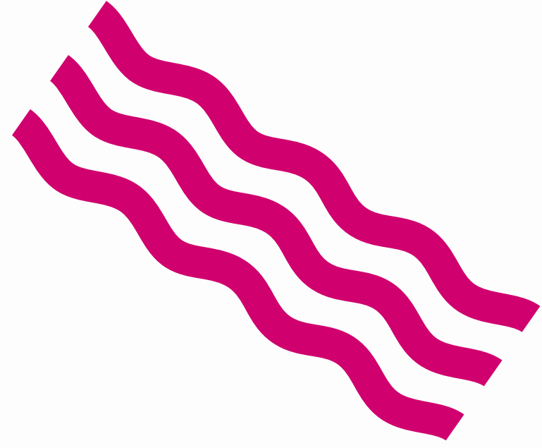
Gravitational Waves
