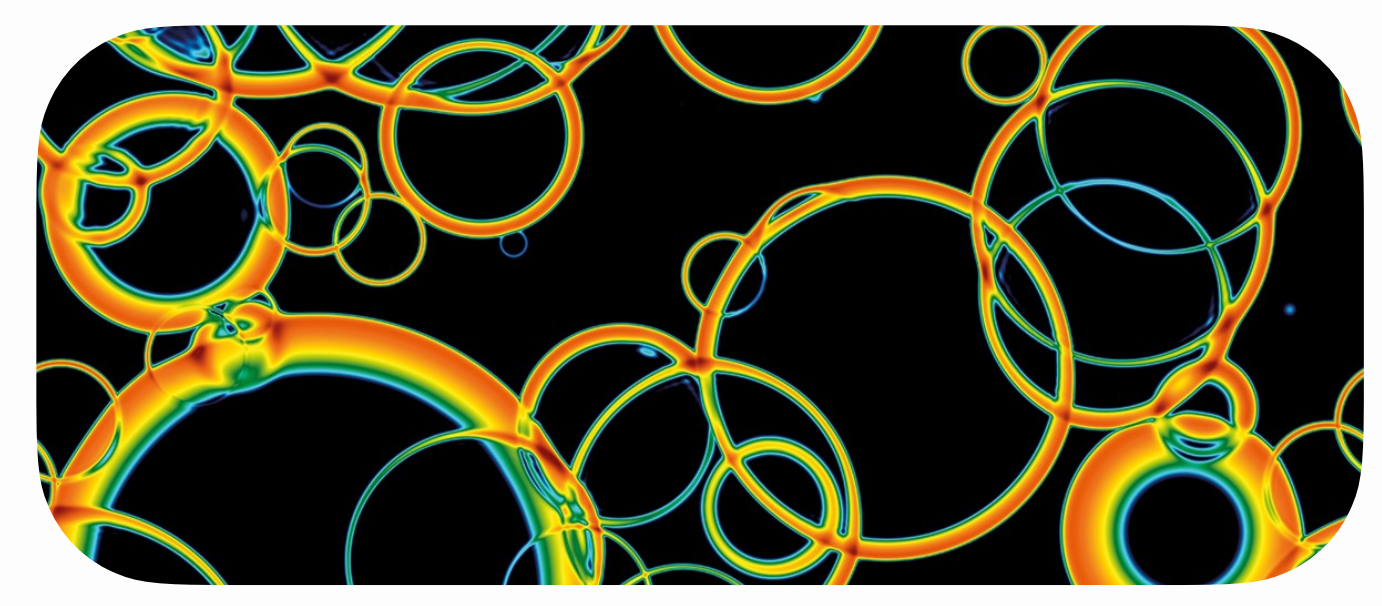
Phase transitions
