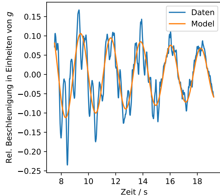
Model vs. Daten
